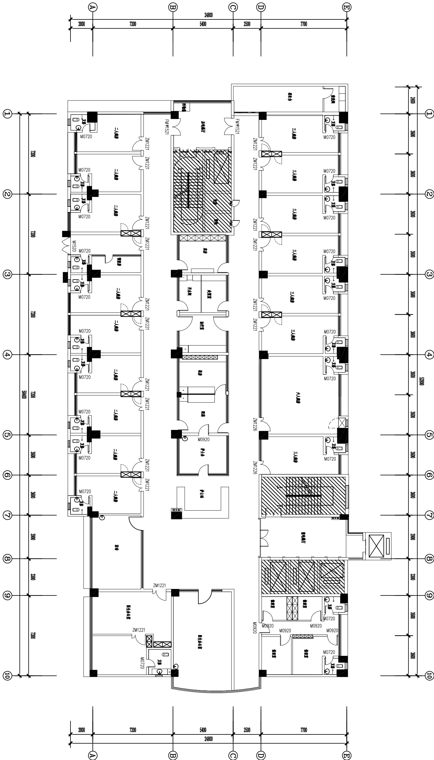
ARCHITECTURAL INFO. PLAN 人医住院楼三楼普外科原状平面图 SCALE 1:200
