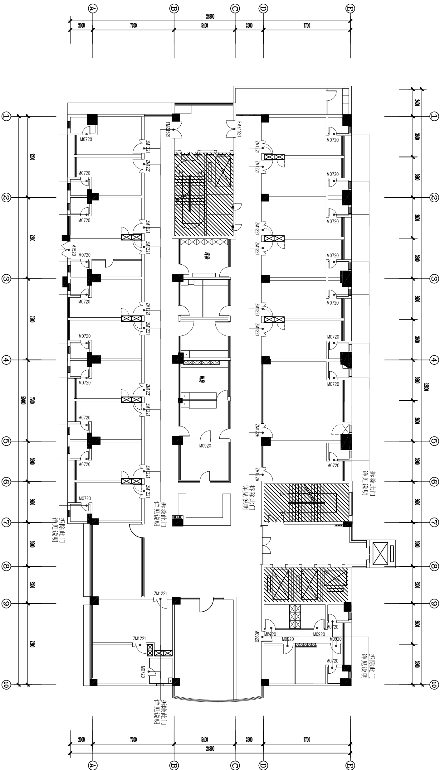
ARCHITECTURAL INFO. PLAN 人医住院楼三楼普外科拆门平面图 SCALE 1:200
